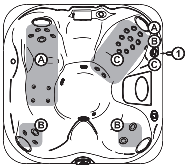
Massage Selector #1 Controls the Main Pump's Water Flow.
